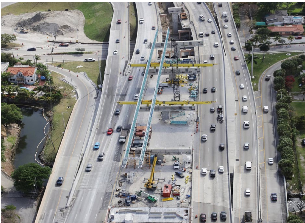
Ongoing assembly of the specialized cap/beam lifter that will erect bridge caps and beams for the new double decked section of SR 836
