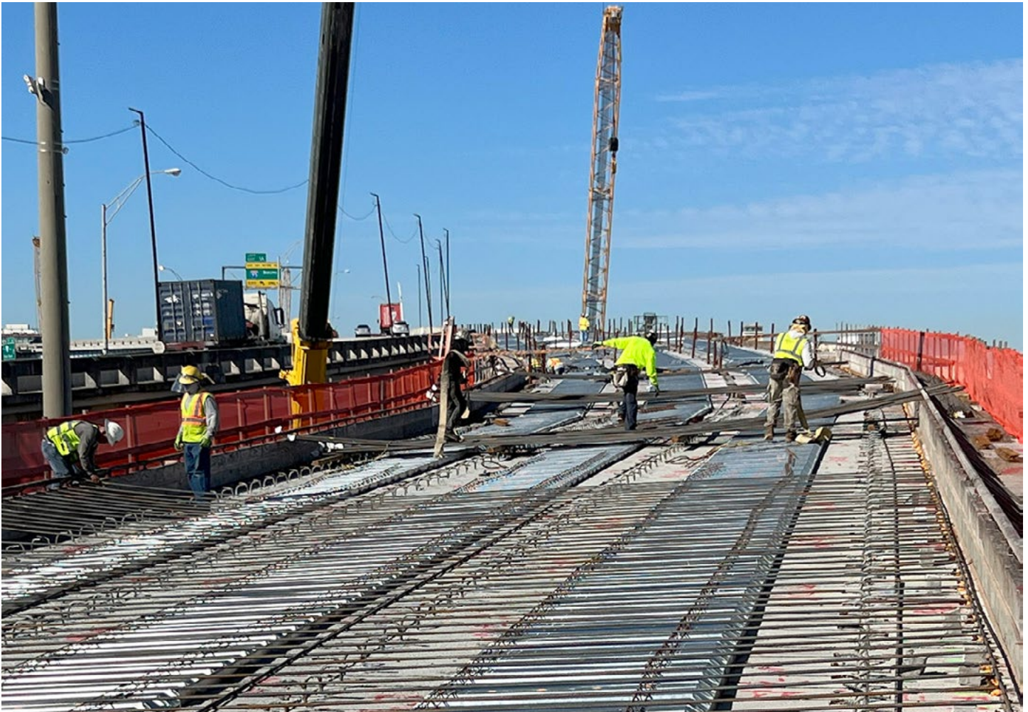
Installation of reinforcing steel at the temporary I-395 bridge that will drivers to SR 836 and southbound I-95
