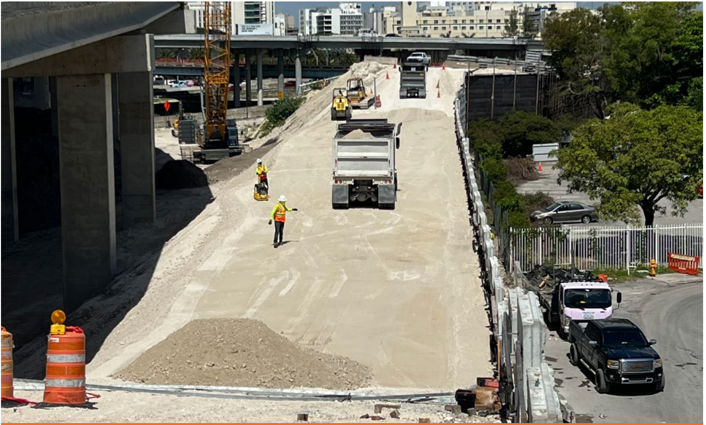
Construction of permanent ramp from westbound I-395 to northbound I-95
